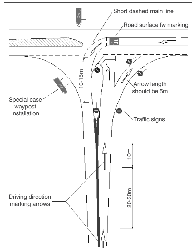
Figure 2 - Recommended signing and marking layout on the intersection of the slip road and a minor road
