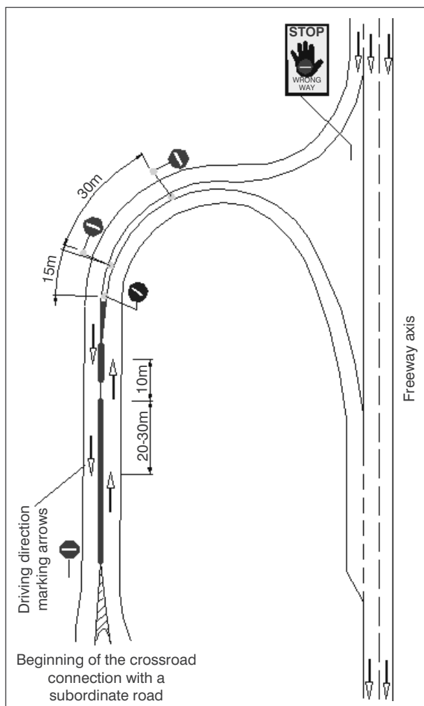
Figure 1 - Recommended signing and road markings on slip and exit roads
