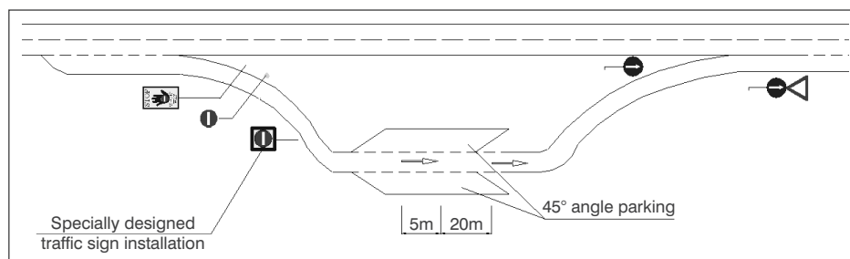
Figure 3 - Recommended signing and marking layout at service stations and petrol services
